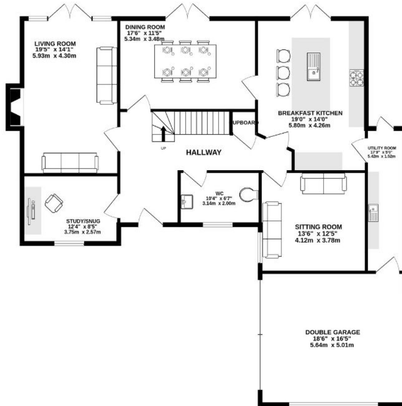
GROUND FLOOR 1623 sq.ft. (150.7 sq.m.) approx.
